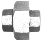
GP104 Galvanized Union (Brass to Iron Seat)- FPT x FPT
